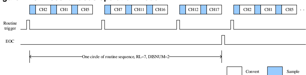
Figure 12-6. Discontinuous operation mode
