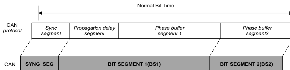
Figure 21-11. The bit time
