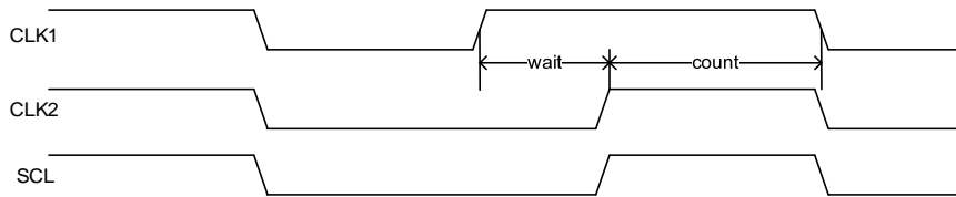
Figure 17-4. Clock synchronization
