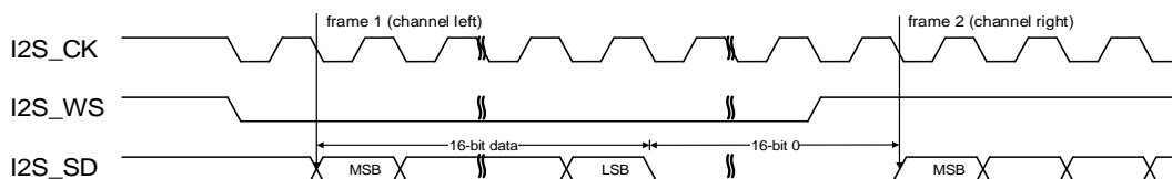
Figure 18-25. I2S Philips standard timing diagram (DTLEN=00, CHLEN=1, CKPL=1)
