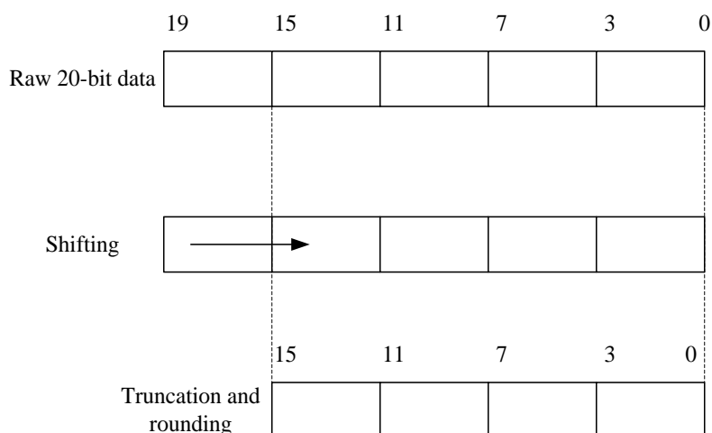
Figure 10-11. 20-bit to 16-bit result truncation
