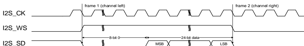
Figure 18-34. LSB justified standard timing diagram (DTLEN=01, CHLEN=1, CKPL=0)
