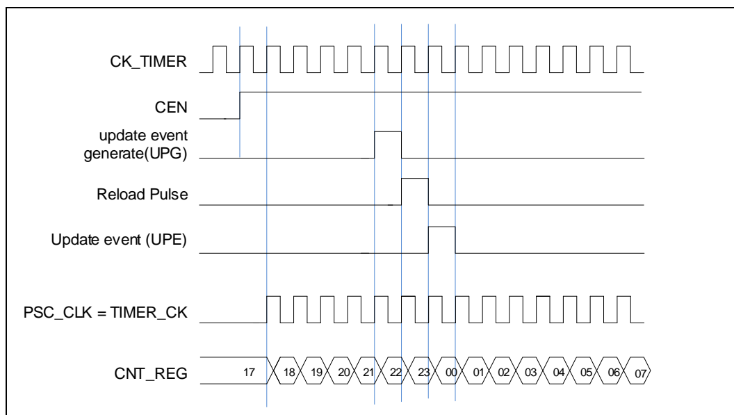
Figure 14-45. Timing chart of internal clock divided by 1
