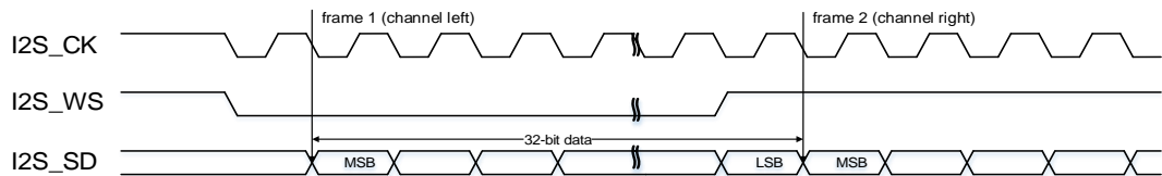
Figure 18-21. I2S Philips standard timing diagram (DTLEN=10, CHLEN=1, CKPL=1)
