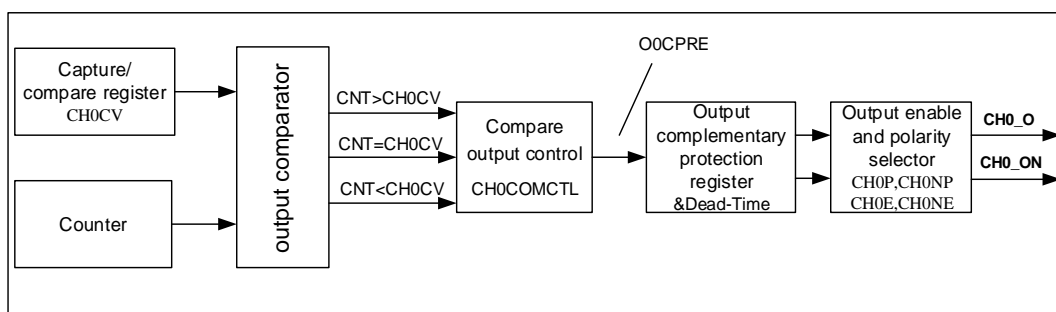
Figure 14-77. Channel output compare principle (with complementary output, x=0)
