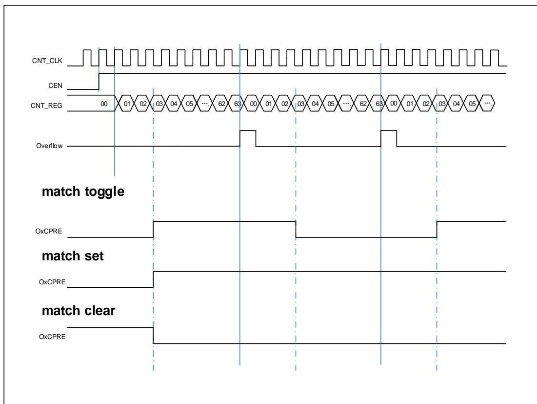
Figure 14-78. Output-compare under three modes
