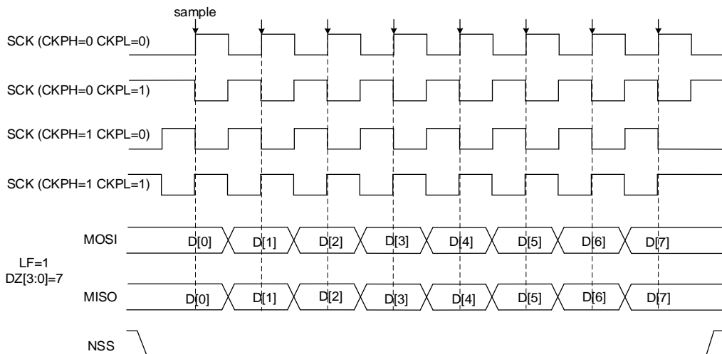
Figure 18-3. SPI1 timing diagram in normal mode
