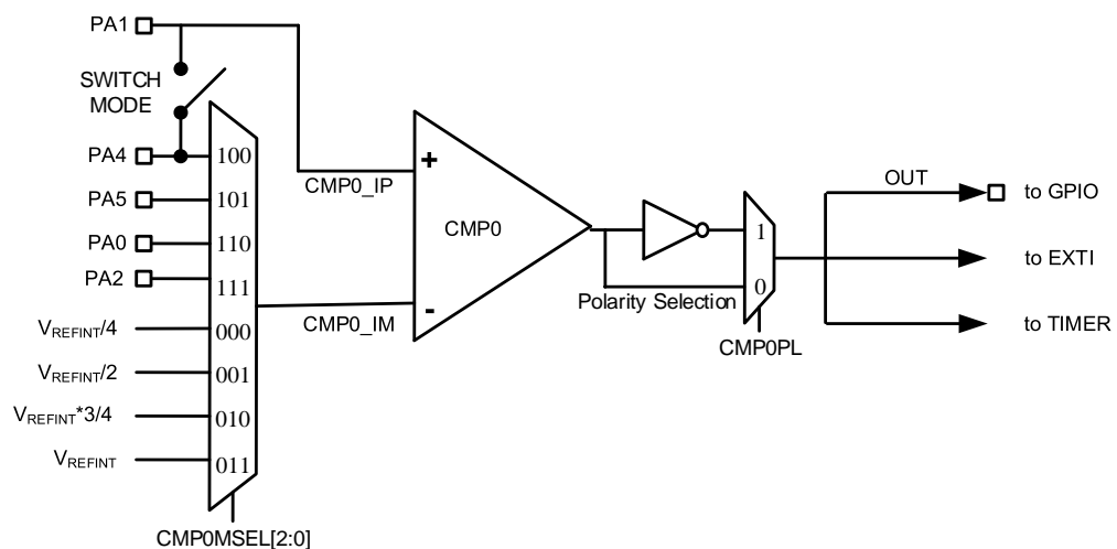
Figure 11-1. CMP block diagram
