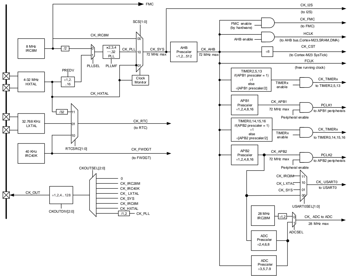
Figure 4-2. Clock tree
