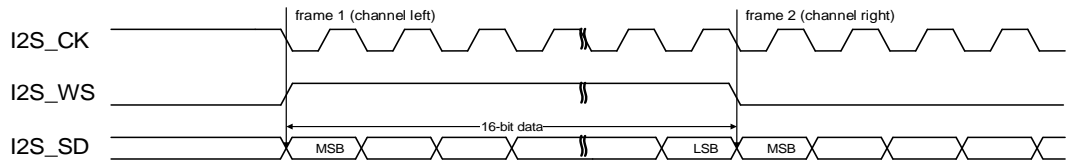
Figure 18-27. MSB justified standard timing diagram (DTLEN=00, CHLEN=0, CKPL=1)
