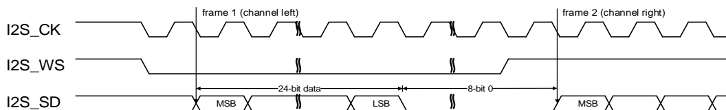
Figure 18-23. I2S Philips standard timing diagram (DTLEN=01, CHLEN=1, CKPL=1)
