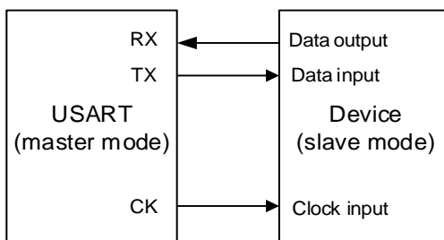
Figure 16-11. Example of USART in synchronous mode
