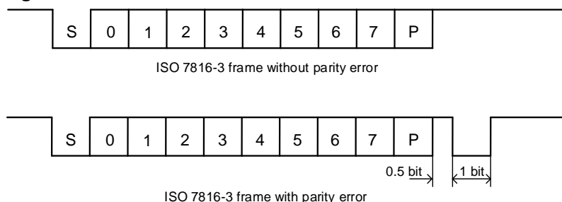
Figure 16-15. ISO7816-3 frame format
