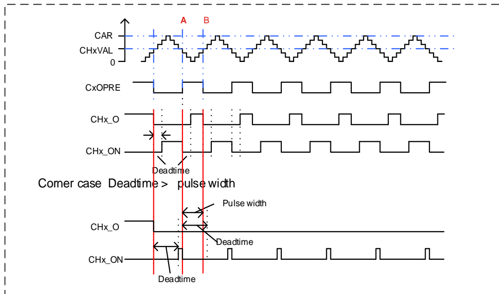
Figure 14-64. Complementary output with dead-time insertion.
