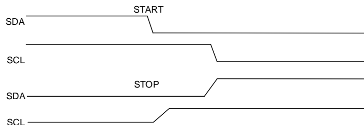
Figure 17-3. START and STOP signal
