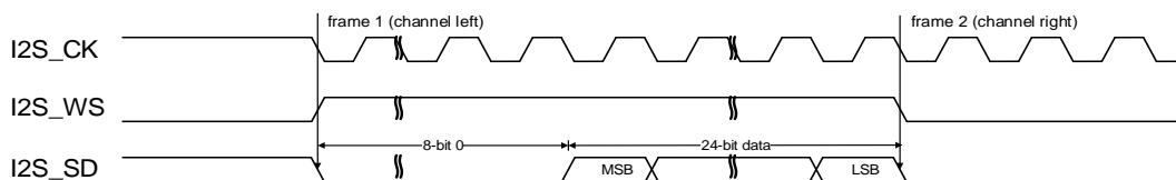
Figure 18-35. LSB justified standard timing diagram (DTLEN=01, CHLEN=1, CKPL=1)
