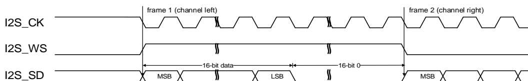
Figure 18-33. MSB justified standard timing diagram (DTLEN=00, CHLEN=1, CKPL=1)
