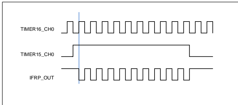
Figure 15-1. IFRP output timechart 1
