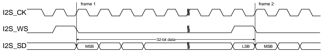
Figure 18-41. PCM standard short frame synchronization mode timing diagram (DTLEN=10, CHLEN=1, CKPL=1)
