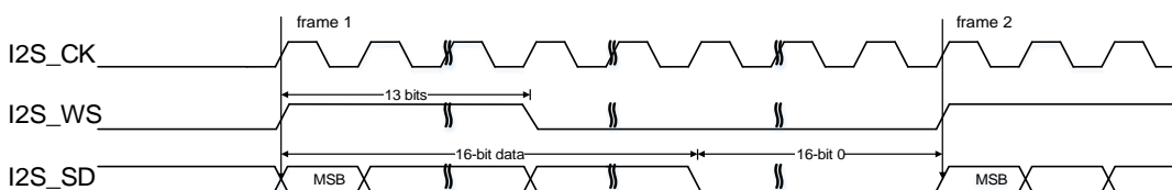
Figure 18-52. PCM standard long frame synchronization mode timing diagram (DTLEN=00, CHLEN=1, CKPL=0)
