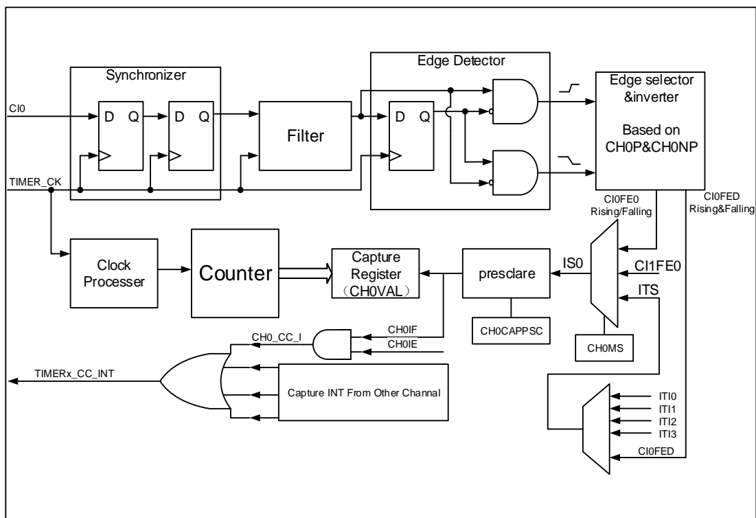
Figure 14-76. Channel input capture principle
