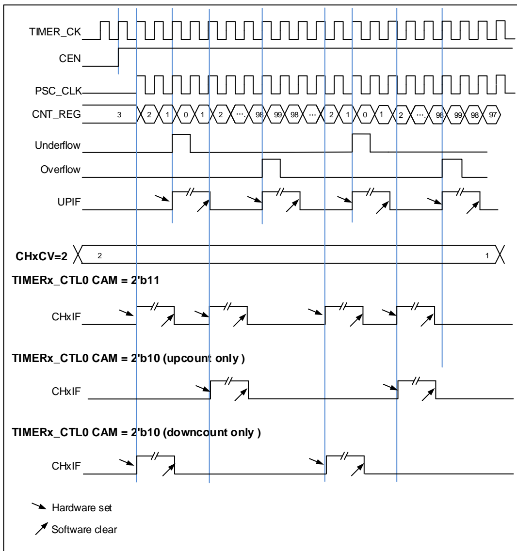
Figure 14-38. Timing chart of center-aligned counting mode
