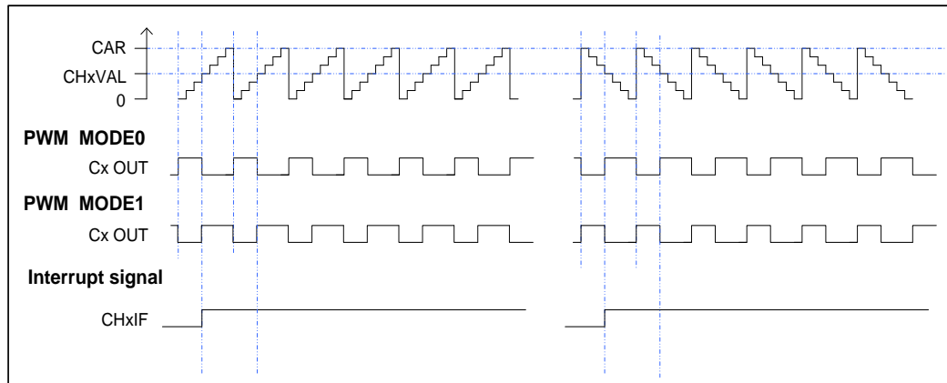
Figure 14-16. Timing chart of EAPWM
