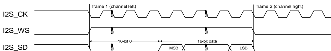
Figure 18-37. LSB justified standard timing diagram (DTLEN=00, CHLEN=1, CKPL=1)
