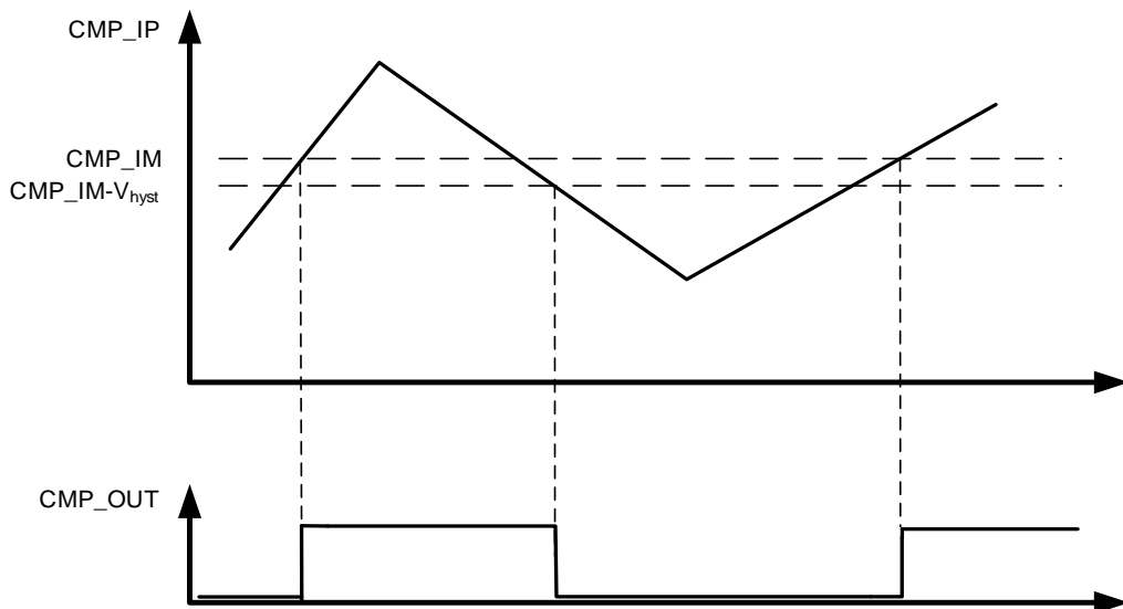
Figure 11-2. CMP hysteresis
