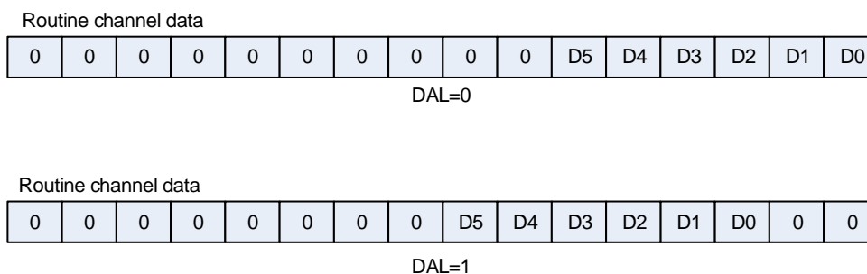
Figure 10-10. Data storage mode of 6-bit resolution
