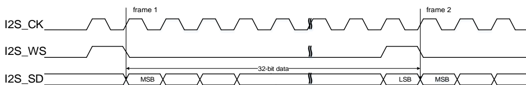
Figure 18-40. PCM standard short frame synchronization mode timing diagram (DTLEN=10, CHLEN=1, CKPL=0)
