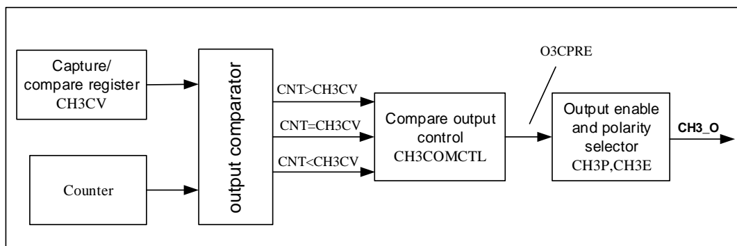
Figure 14-14. Channel output compare principle (CH3_O)
