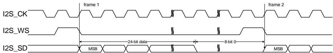
Figure 18-43. PCM standard short frame synchronization mode timing diagram (DTLEN=01, CHLEN=1, CKPL=1)
