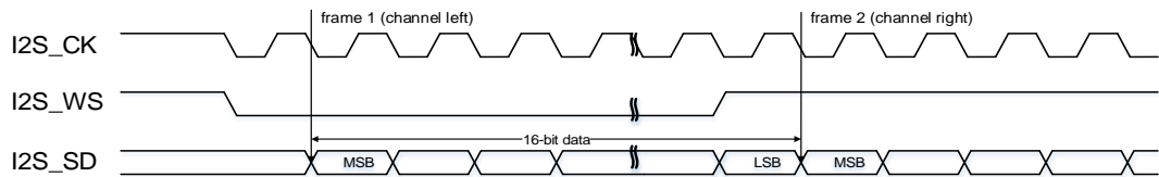
Figure 18-19. I2S Philips standard timing diagram (DTLEN=00, CHLEN=0, CKPL=1)
