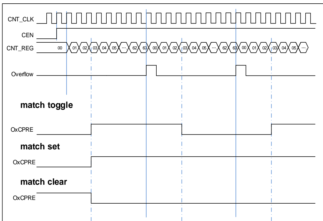
Figure 14-15. Output-compare in three modes
