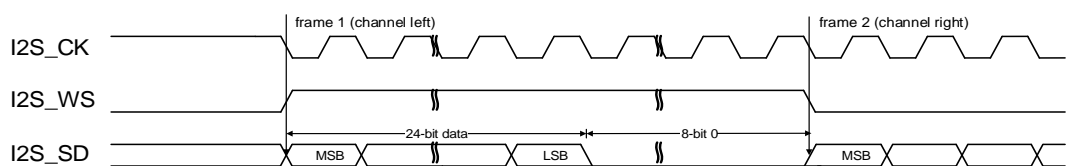
Figure 18-31. MSB justified standard timing diagram (DTLEN=01, CHLEN=1, CKPL=1)
