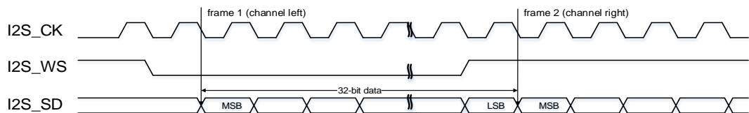
Figure 18-20. I2S Philips standard timing diagram (DTLEN=10, CHLEN=1, CKPL=0)
