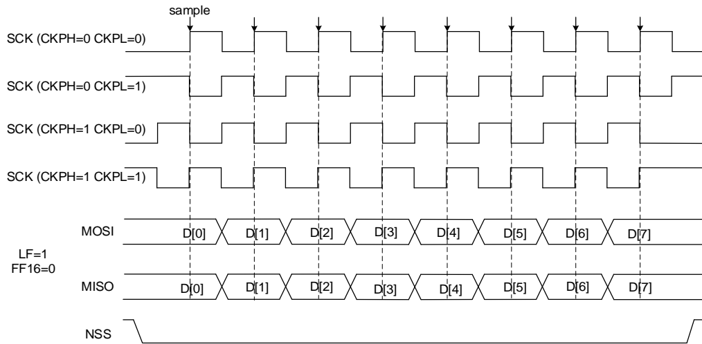
Figure 18-2. SPI0 timing diagram in normal mode
