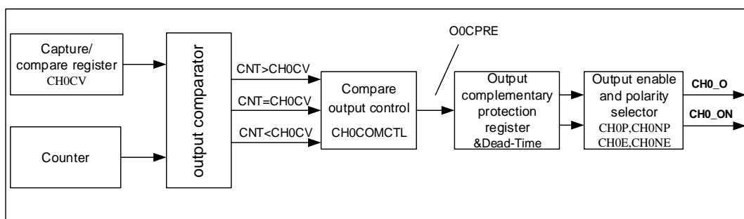
Figure 14-60. Channel output compare principle (with complementary output, x=0)
