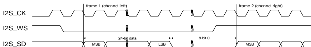
Figure 18-22. I2S Philips standard left timing diagram (DTLEN=01, CHLEN=1, CKPL=0)
