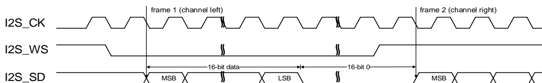
Figure 18-24. I2S Philips standard timing diagram (DTLEN=00, CHLEN=1, CKPL=0)
