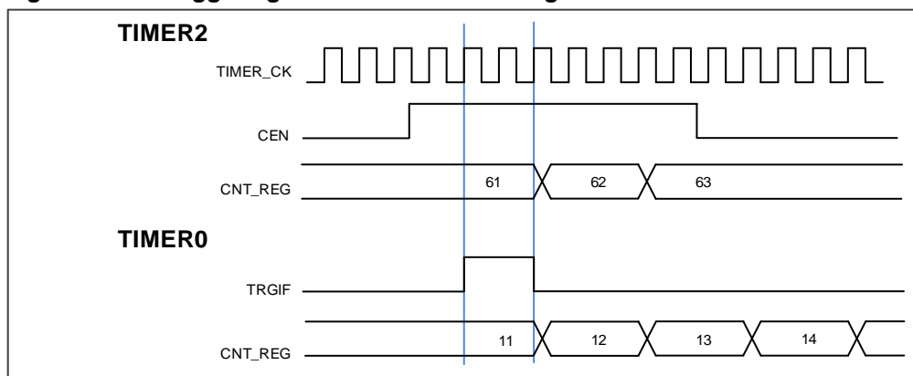
Figure 14-29. Triggering TIMER0 with enable signal of TIMER2
