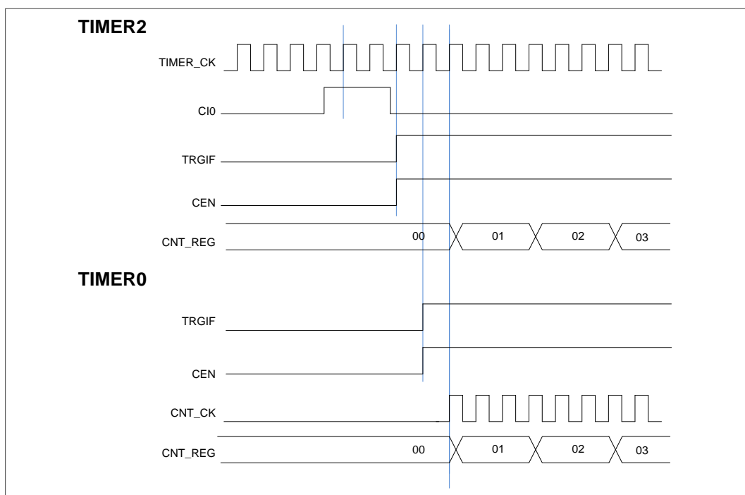
Figure 14-30. Triggering TIMER0 and TIMER2 with TIMER2's CI0 input
