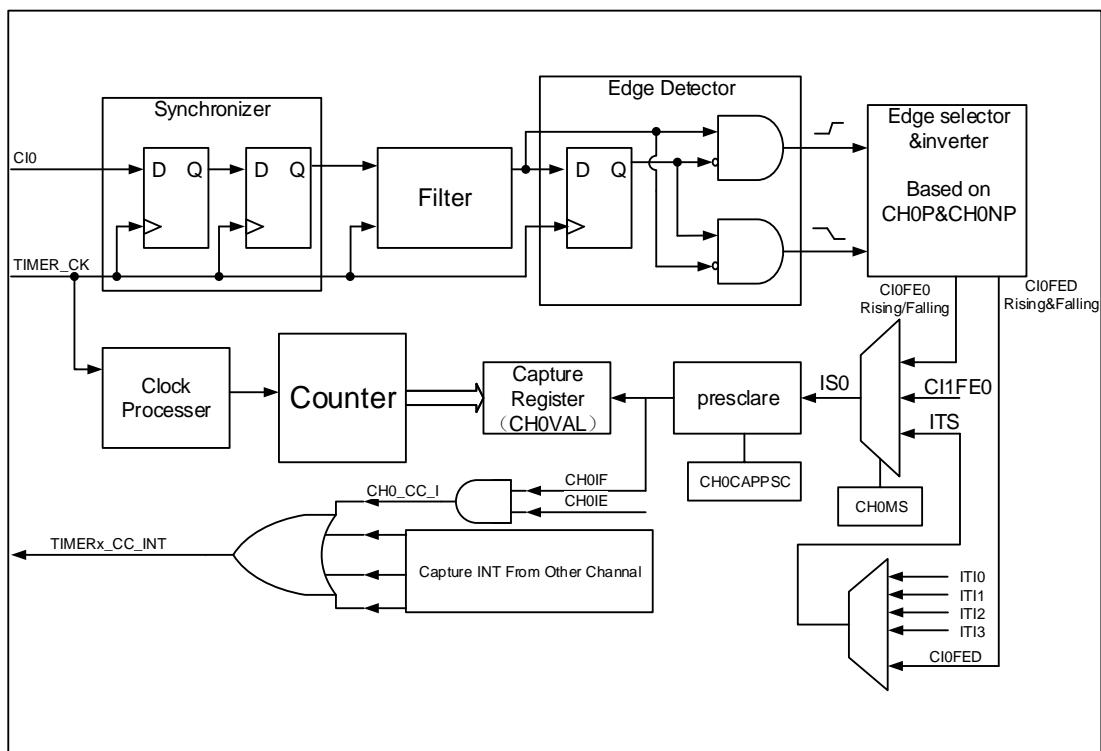
Figure 14-12. Channel input capture principle
