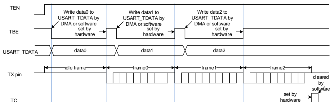
Figure 16-3.USART transmit procedure
