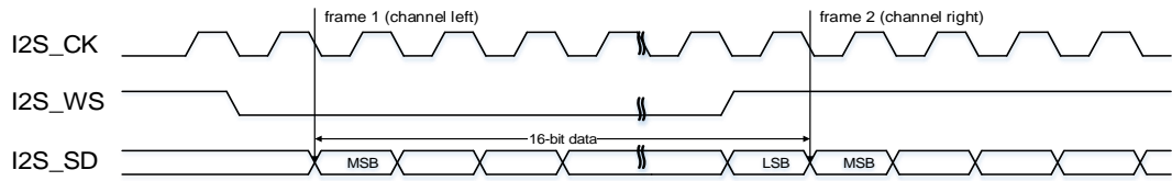
Figure 18-18. I2S Philips standard timing diagram (DTLEN=00, CHLEN=0, CKPL=0)
