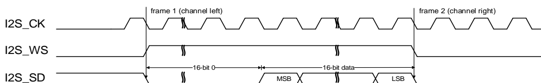
Figure 18-36. LSB justified standard timing diagram (DTLEN=00, CHLEN=1, CKPL=0)
