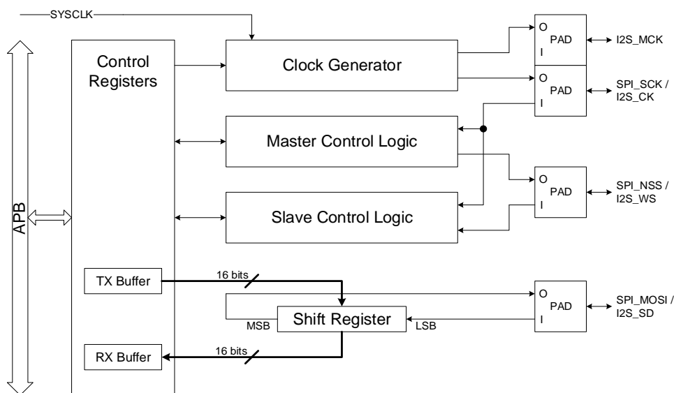
Figure 18-17. Block diagram of I2S
