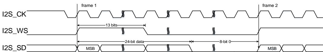
Figure 18-51. PCM standard long frame synchronization mode timing diagram (DTLEN=01, CHLEN=1, CKPL=1)
